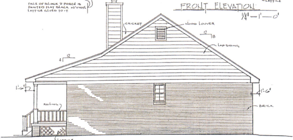
RIGHT SIDE 1/4" = 1'-0"
