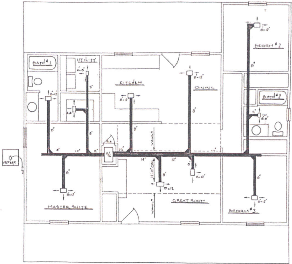
DUCT LAYOUT (SCHEMATIC) 1/4" = 1' = 0"
