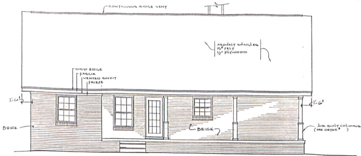
REAR ELEVATION 1/4" = 1'-0"
