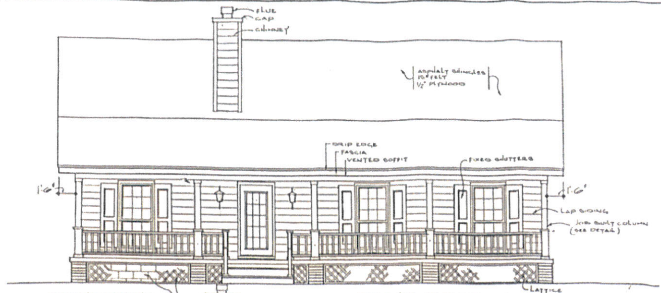
FRONT ELEVATION
