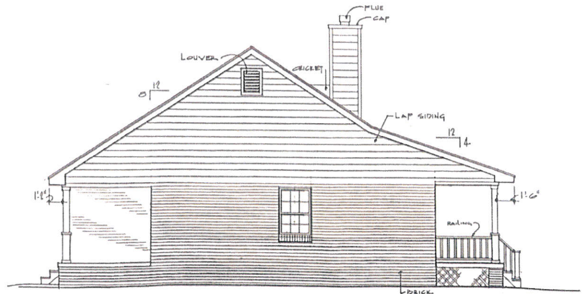
LEFT SIDE 1/4" = 1'-0"
