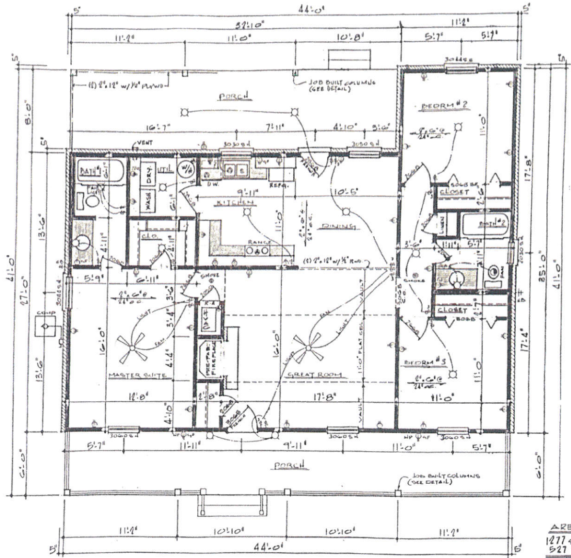
FLOOR PLAN 1/4" = 1'-0"
