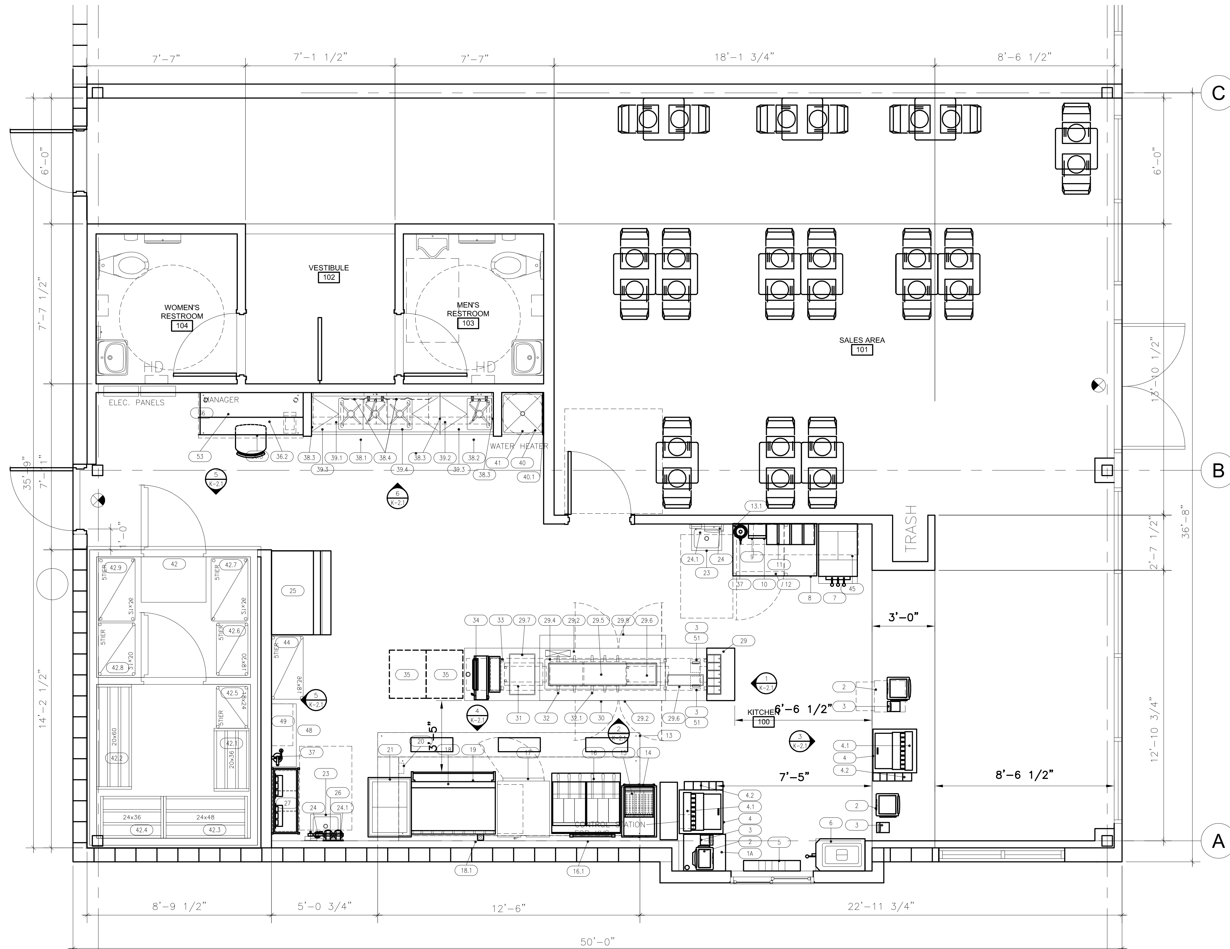
2 EQUIPMENT PLAN SCALE: 3/8" = 1'-0"
